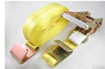
3200 2" RATCHET, 27 FT. WITH 2 FLAT HOOKS RATING: 10,000 LB. BREAKING STRENGTH 3,335 LB. WORKING LOAD
