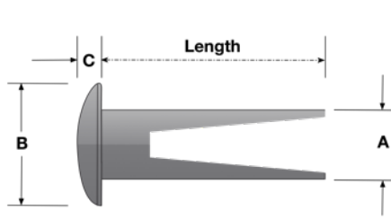
TRUSS HEAD SPLIT RIVET
