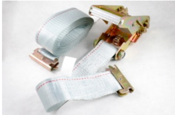
3201 2" RATCHET, 16 FT. WITH E-TRACK FITTINGS RATING: 4,500 LB. BREAKING STRENGTH 1,500 LB. WORKING LOAD
