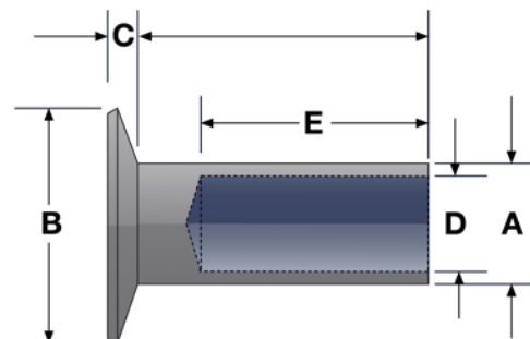
Flat Countersunk Head
